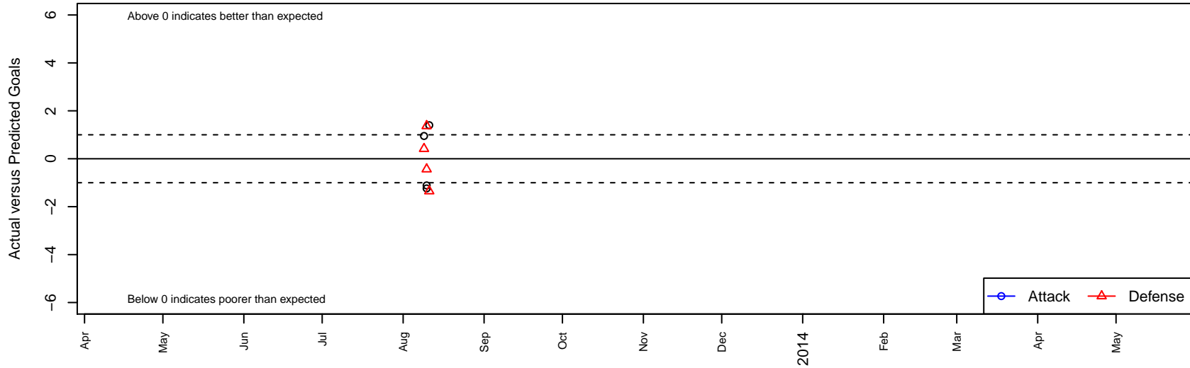
Stevensville Sabres B96 Dots are actual minus expected GF (blue circles) and GA (red triangles). Blue line is smoothed change in attack strength. Red is smoothed change in defense strength.
